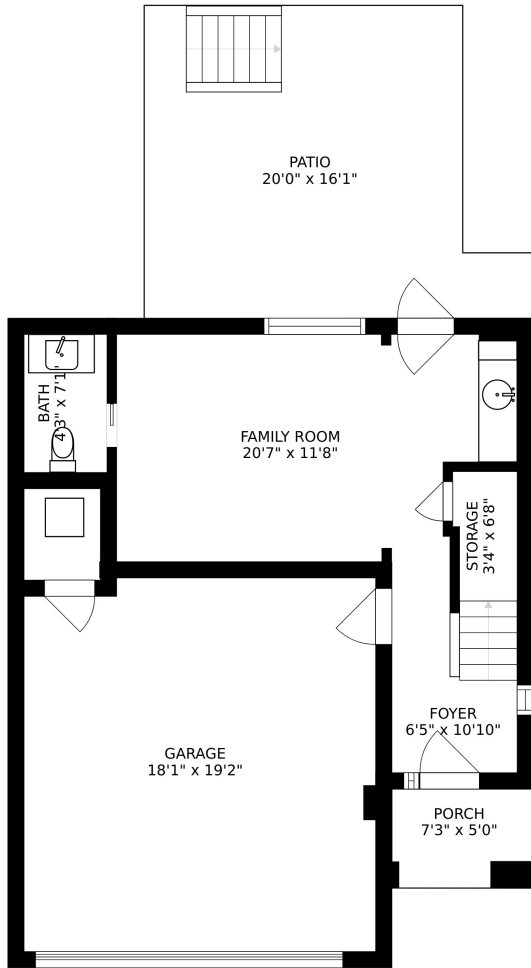
FLOOR 1
