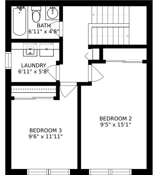
FLOOR 3
