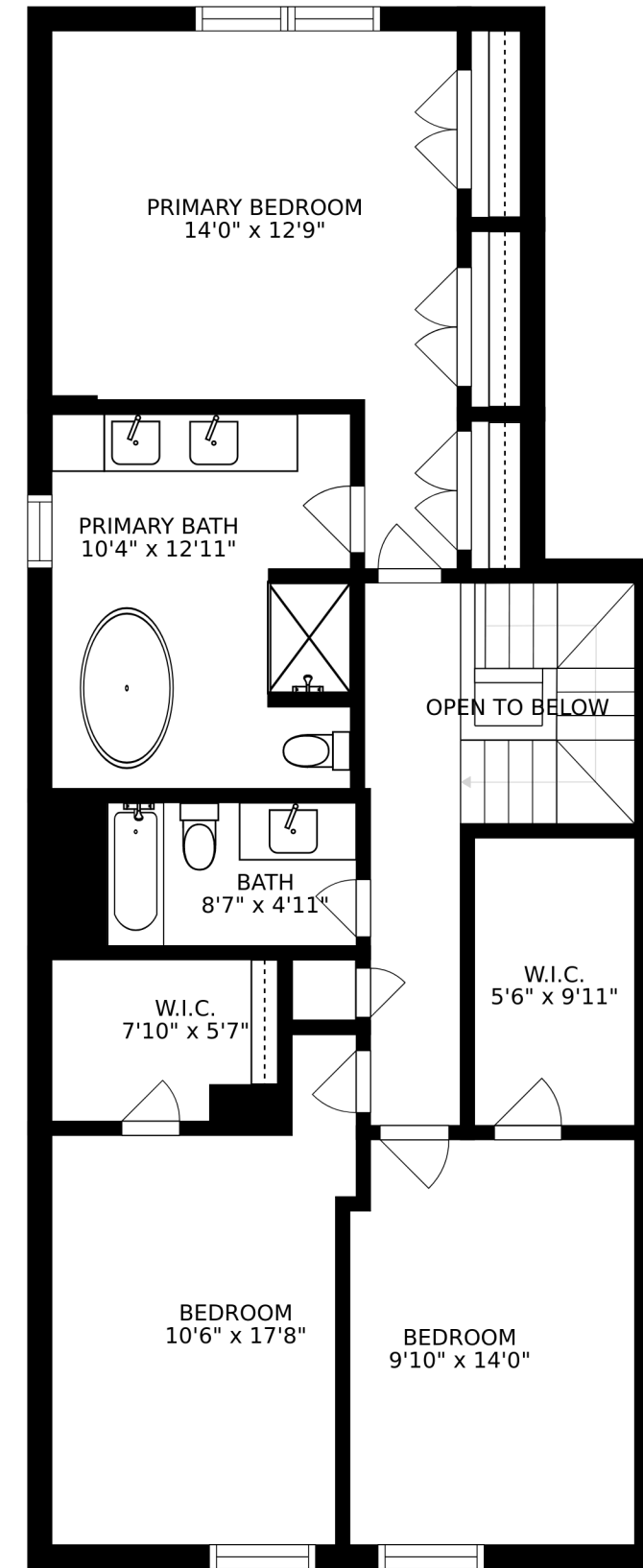
FLOOR 3
