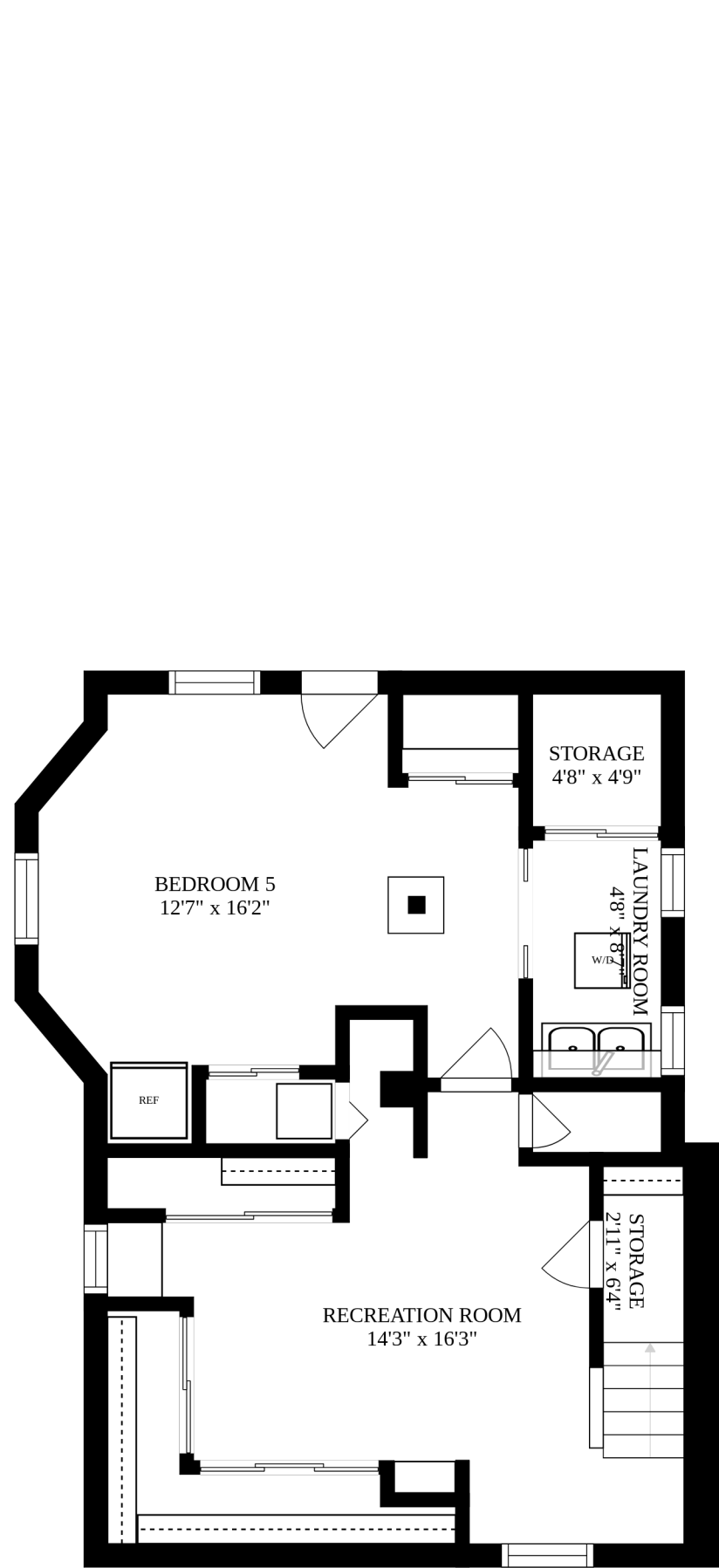
FLOOR 1
