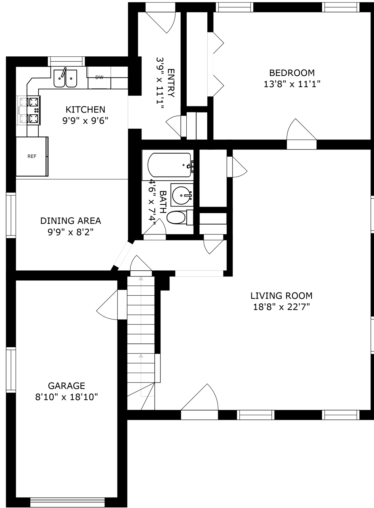
FLOOR 2
