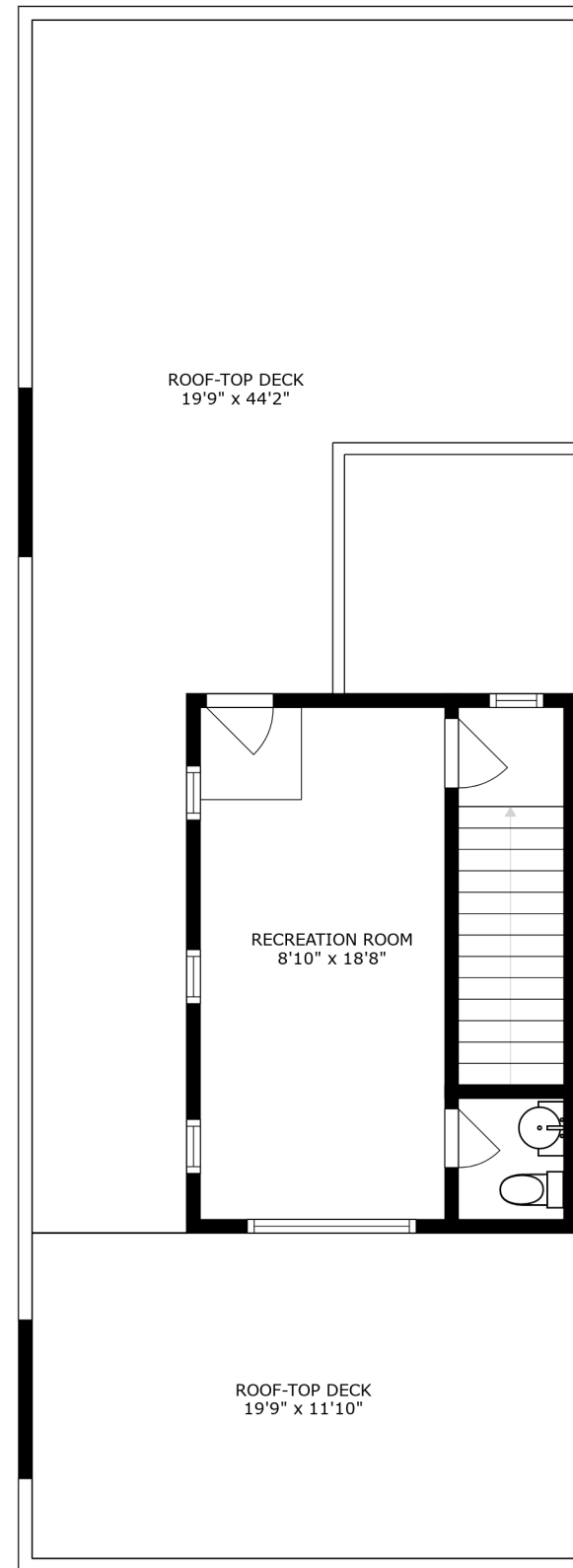
FLOOR 2
