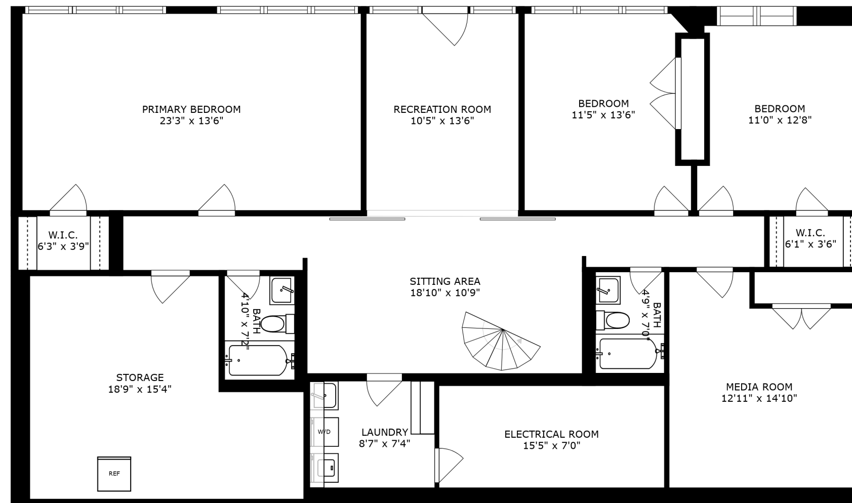
FLOOR 1
