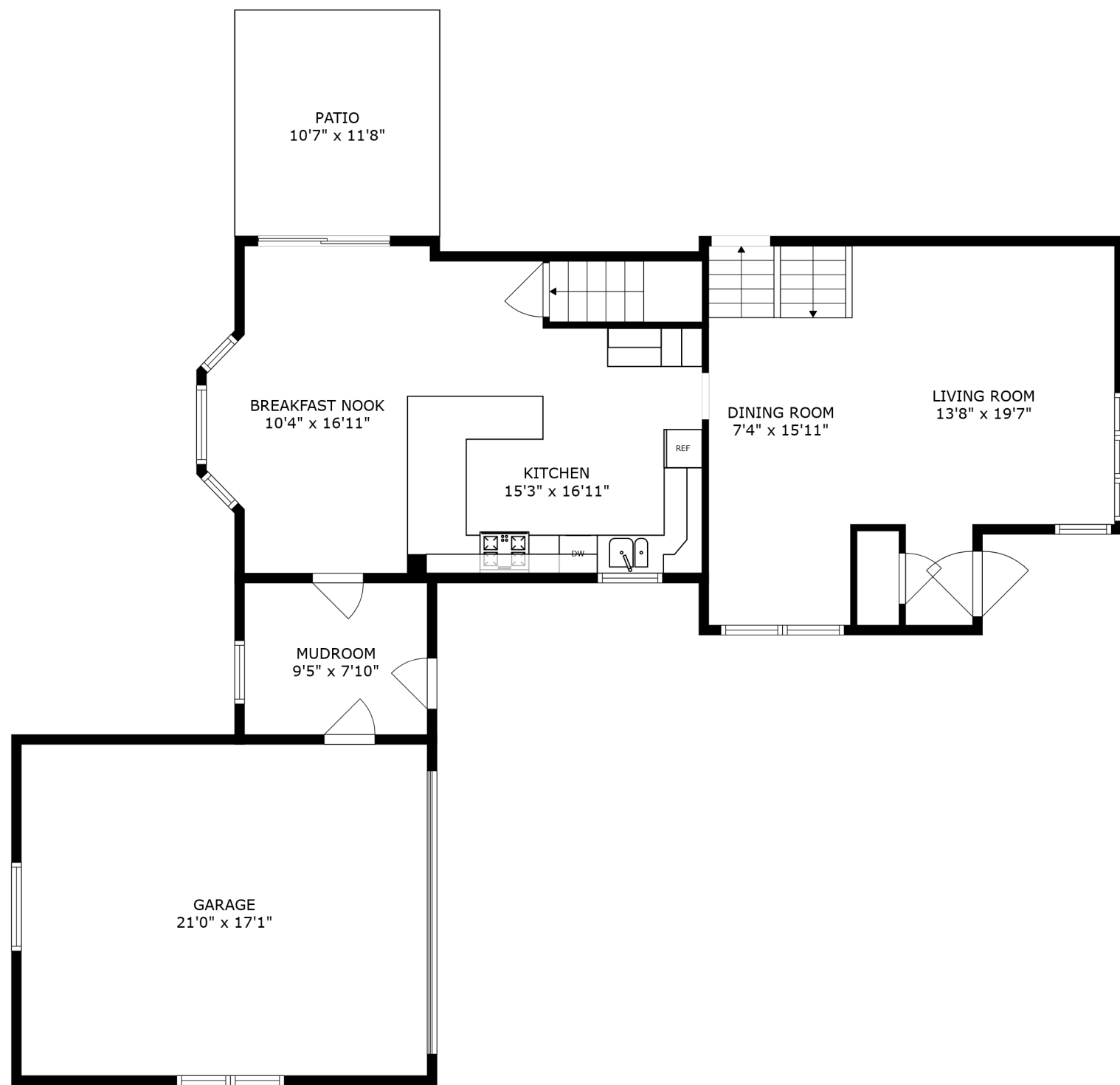
FLOOR 2
