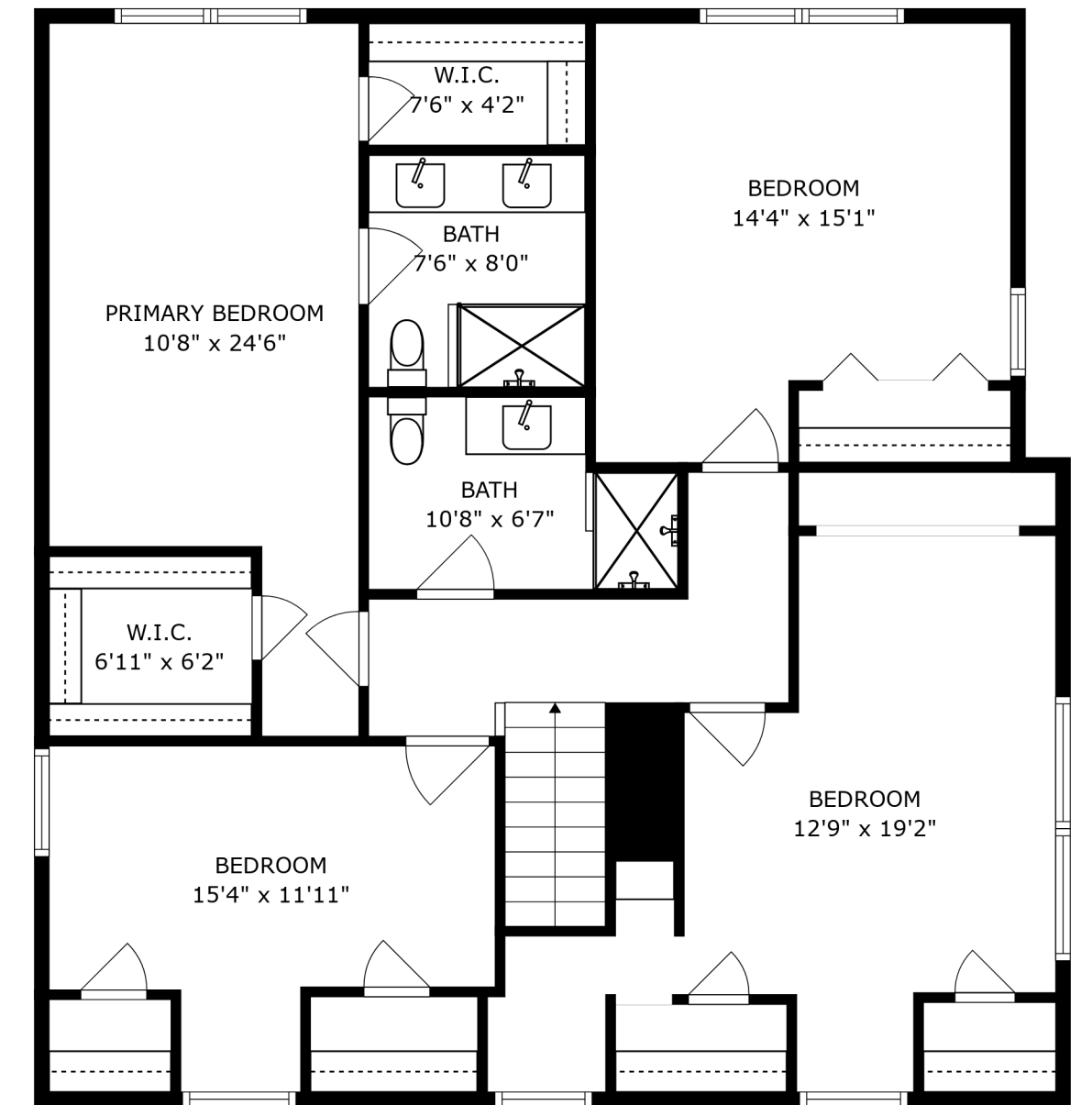
FLOOR 3
