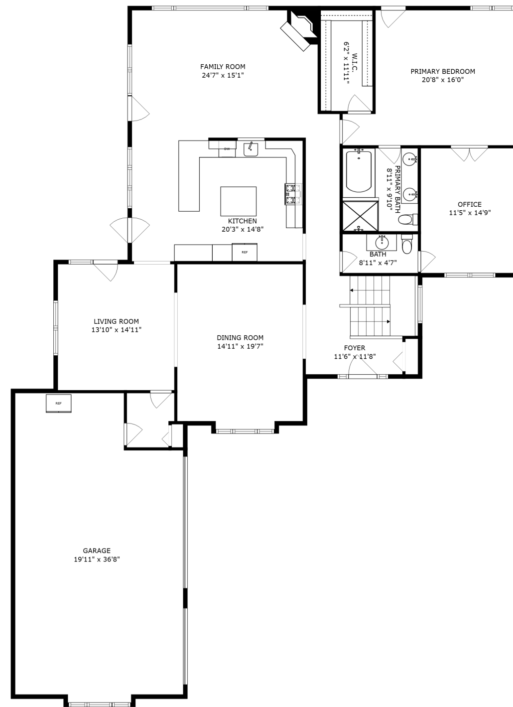
FLOOR 2
