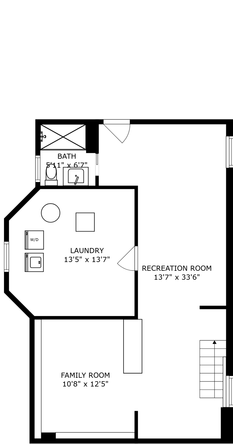
FLOOR 1
