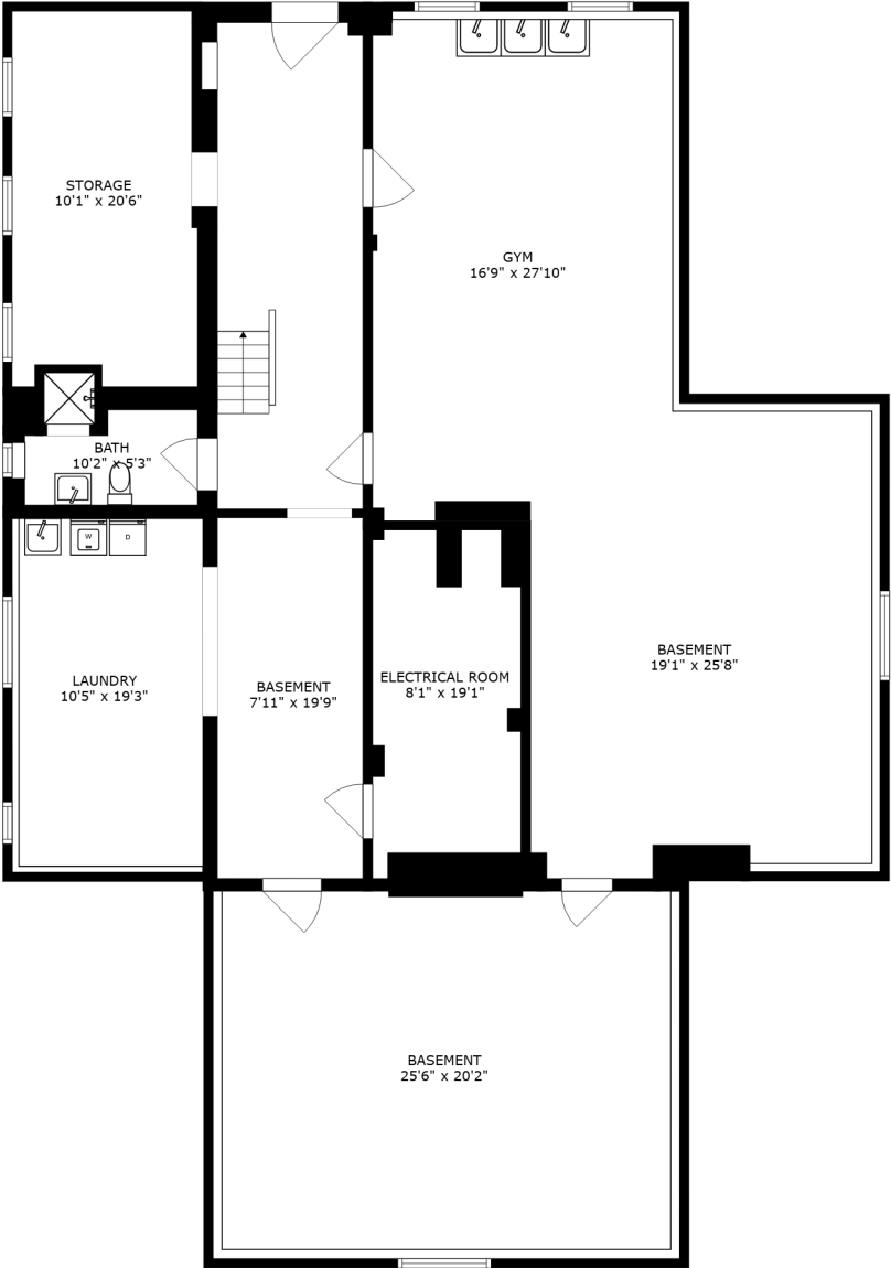
FLOOR 1
