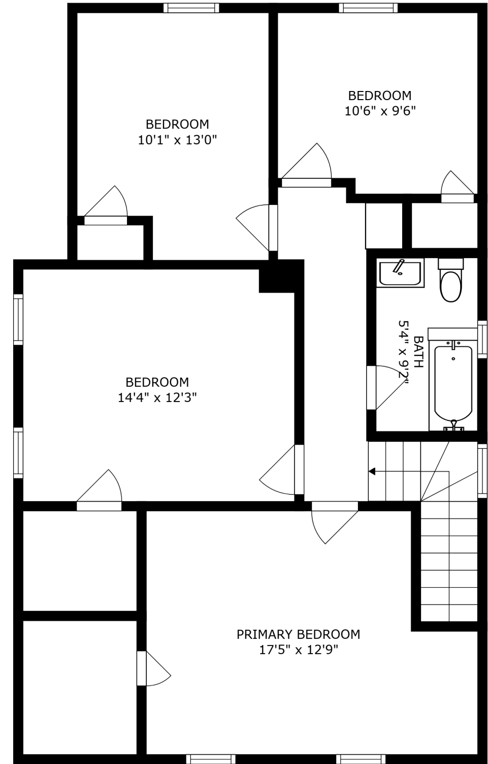
FLOOR 3
