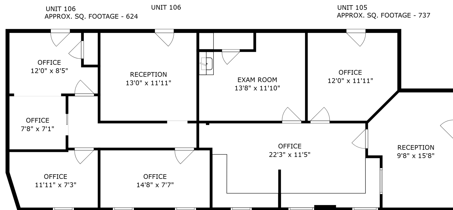
FIRST FLOOR
