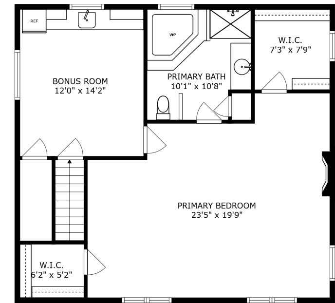
FLOOR 3
