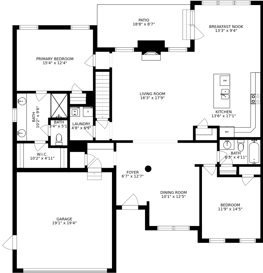
FLOOR 2
