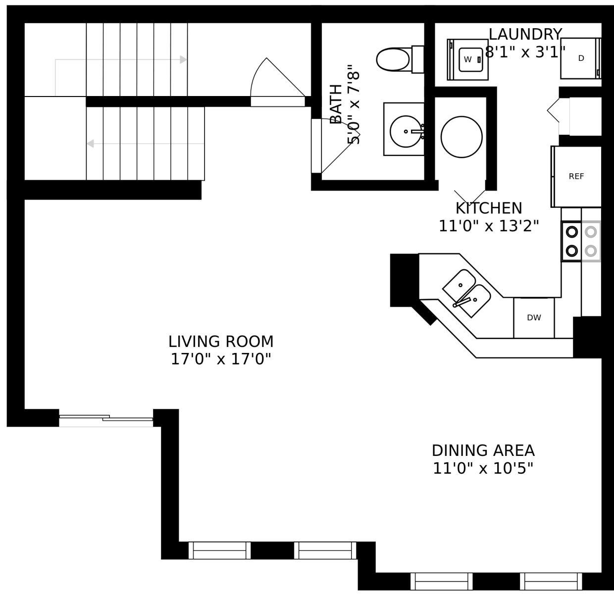
FLOOR 2
