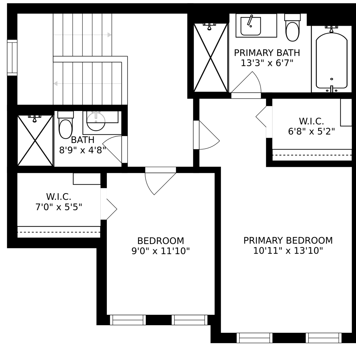
FLOOR 3
