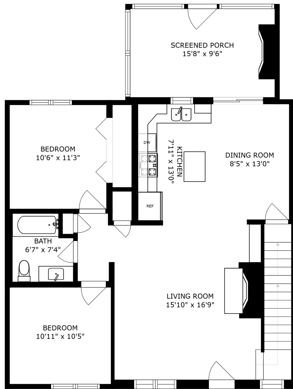
FLOOR 2
