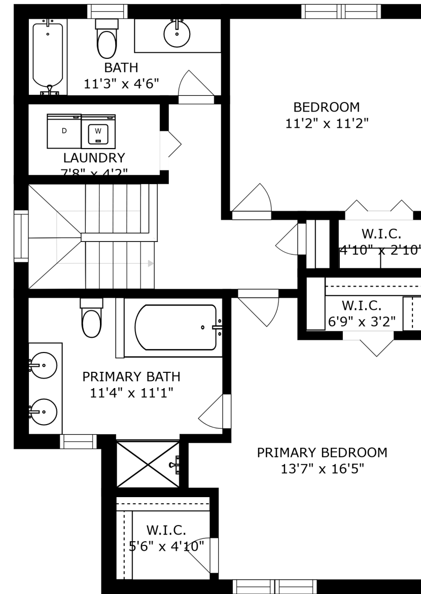
FLOOR 3
