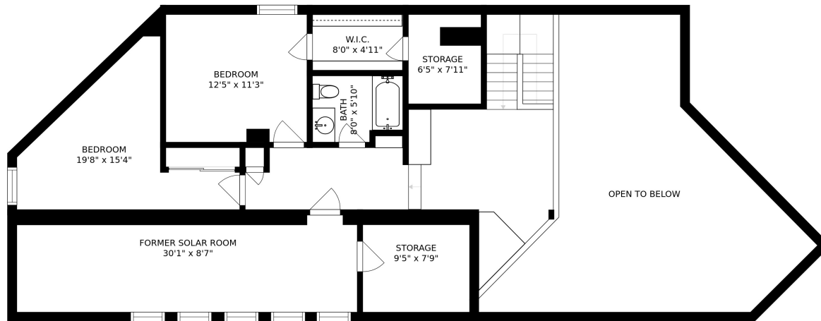
FLOOR 2
