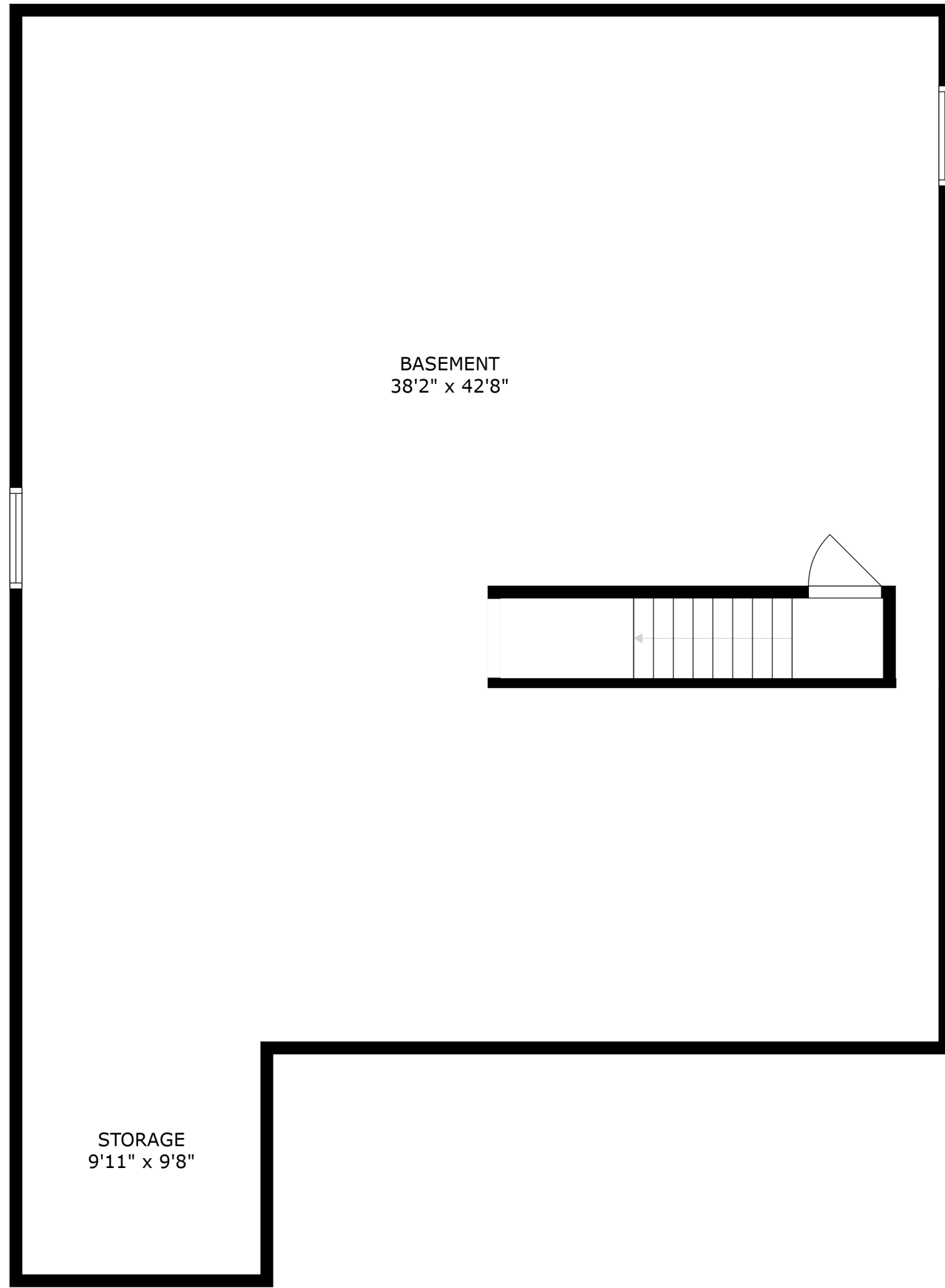
FLOOR 1
