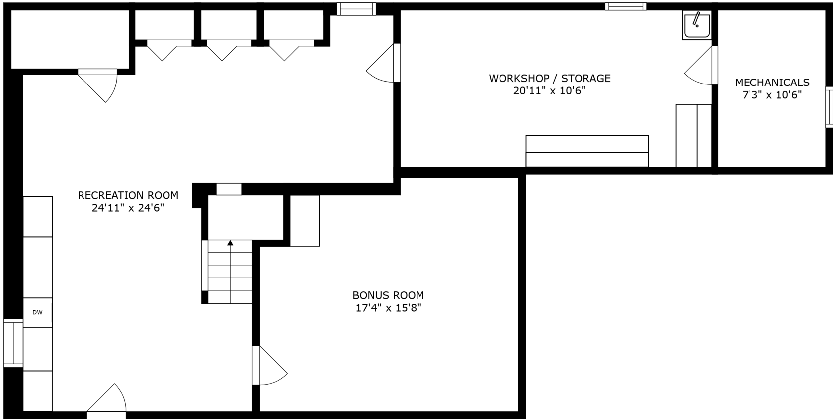
FLOOR 1
