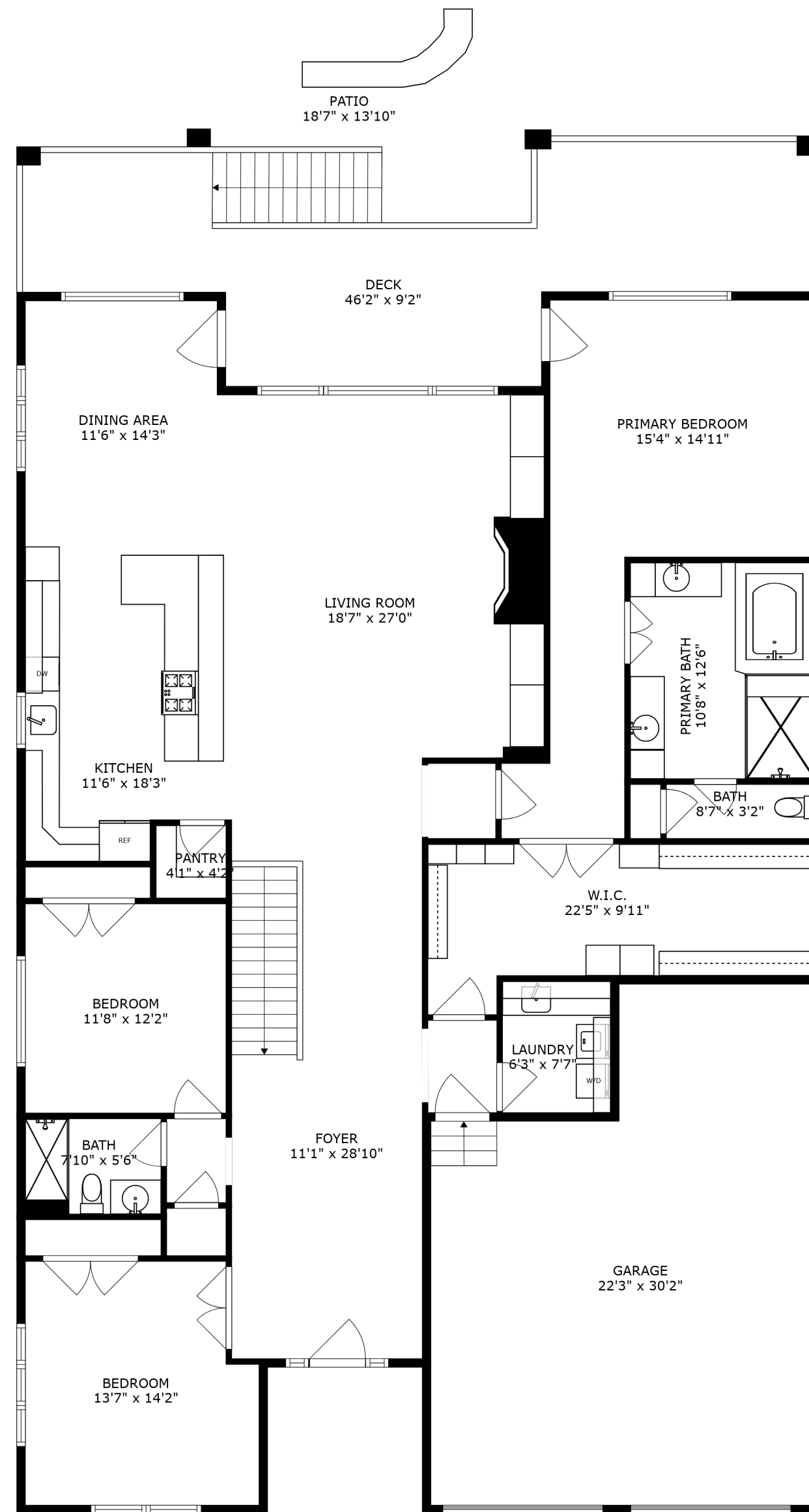
FLOOR 2
