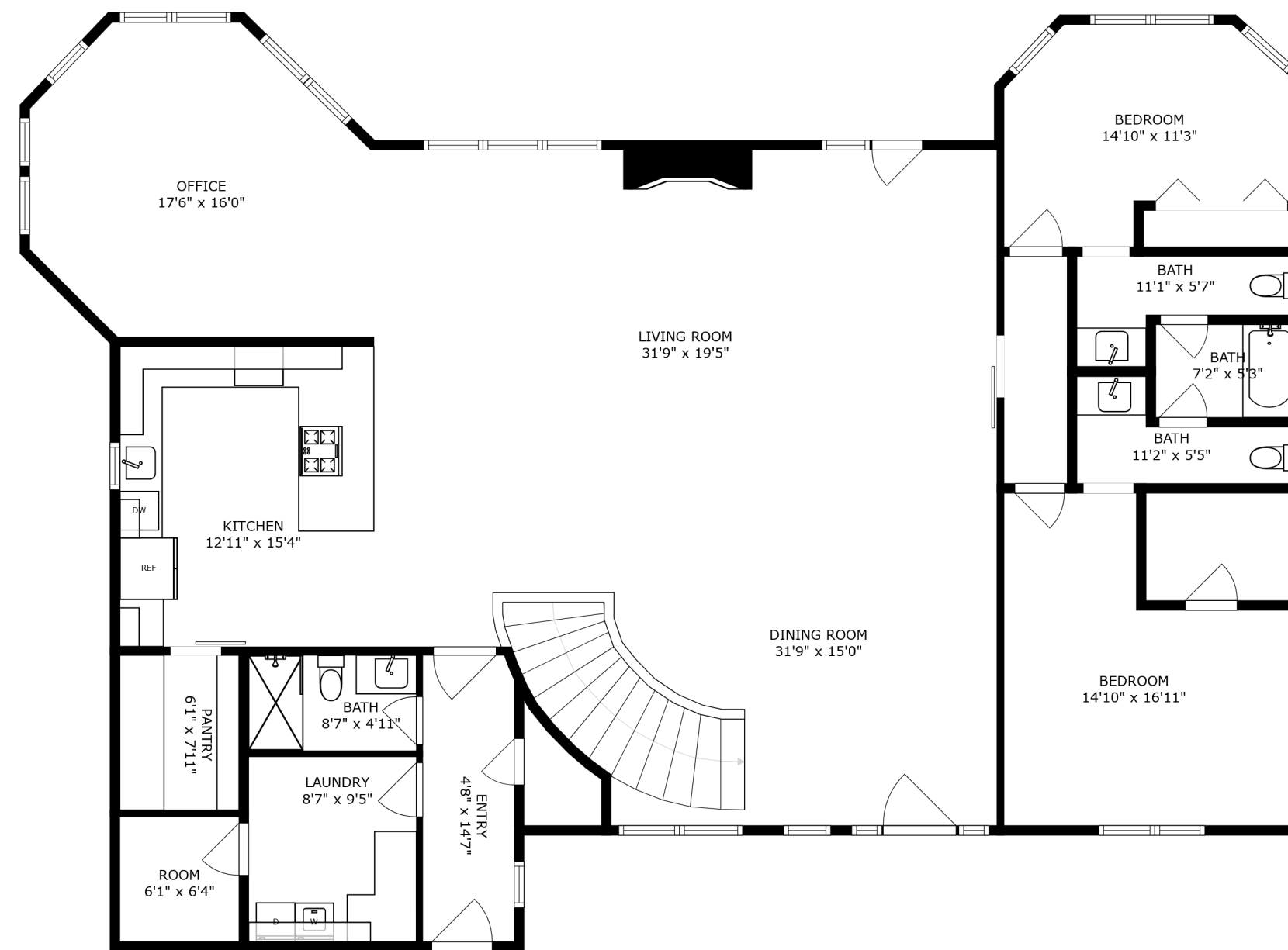
FLOOR 2
