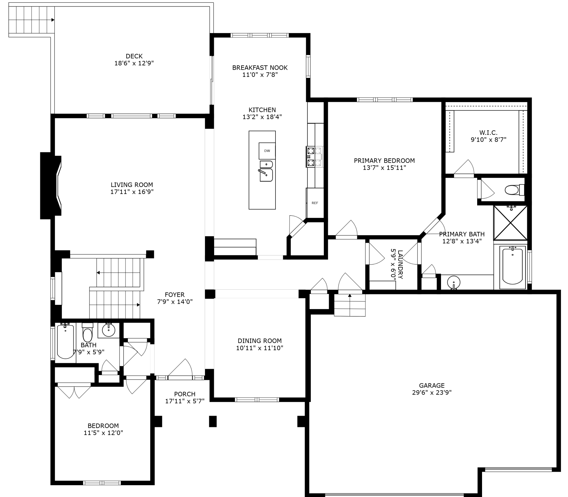
FLOOR 2
