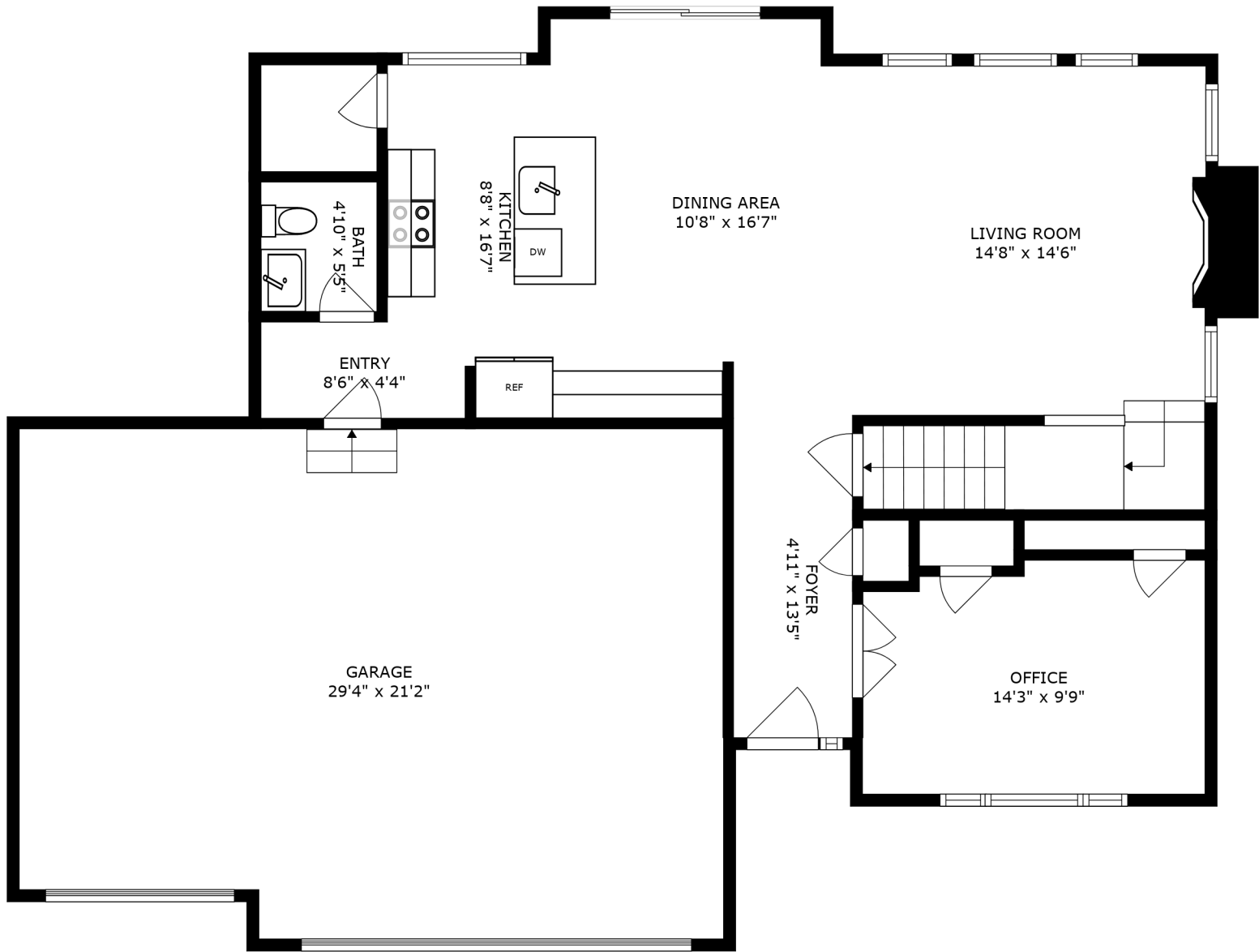
FLOOR 2
