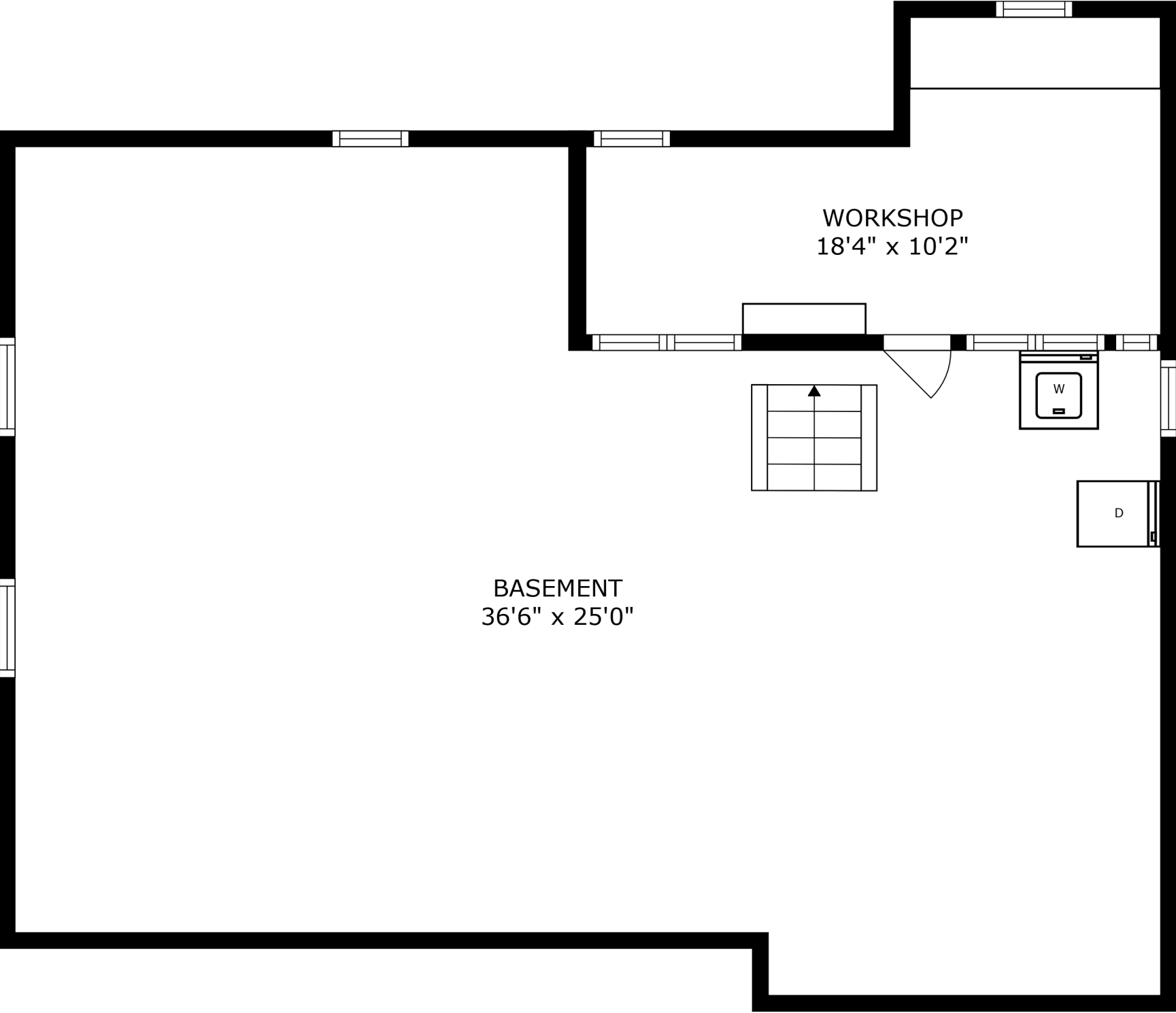
FLOOR 1
