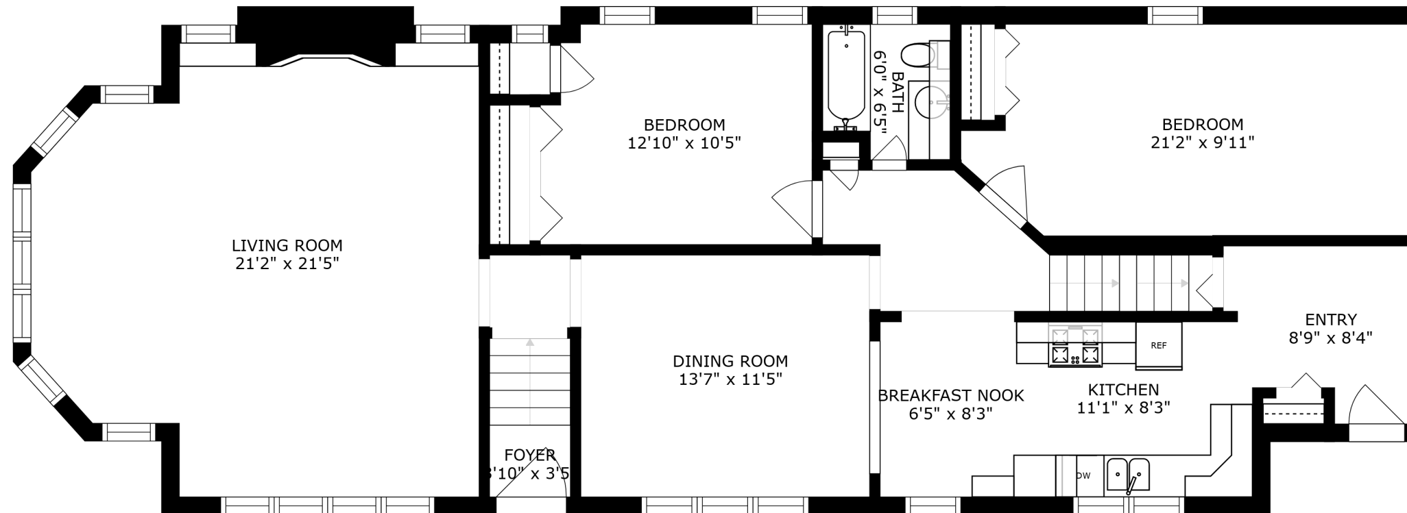
FLOOR 2
