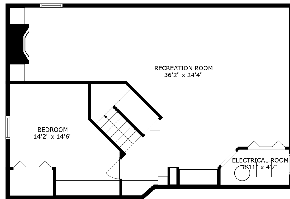
FLOOR 1
