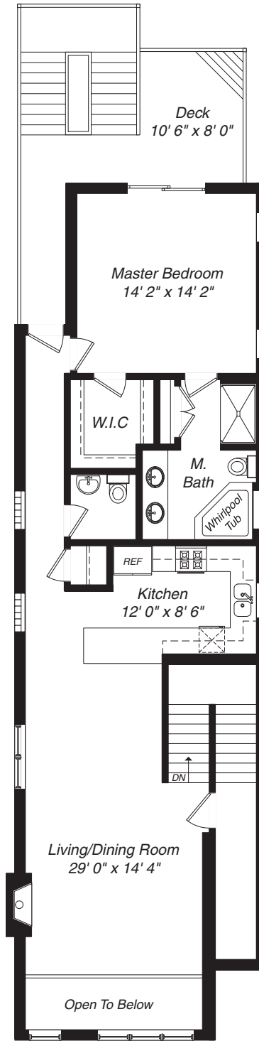
First Floor
