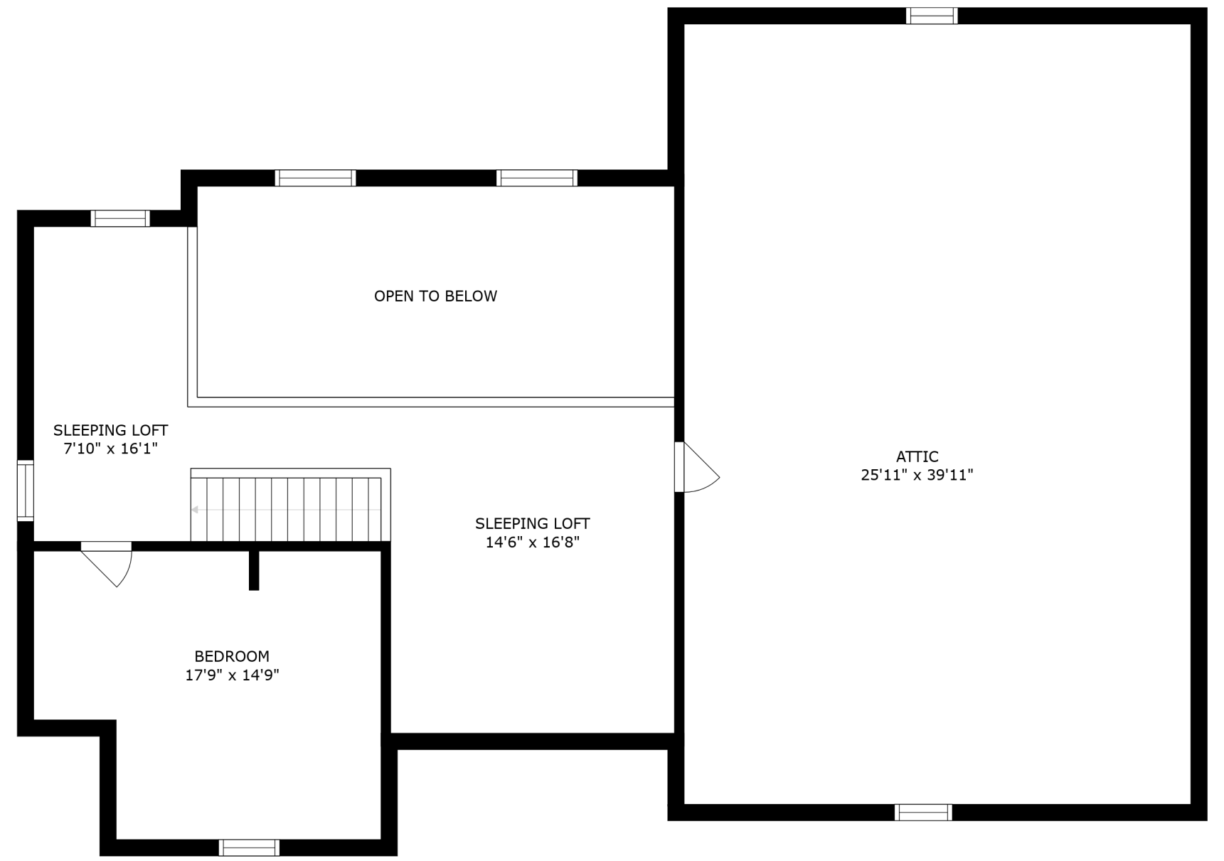
FLOOR 2
