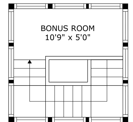
FLOOR 3
