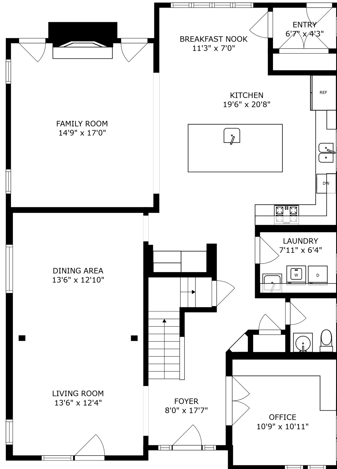
FLOOR 2
