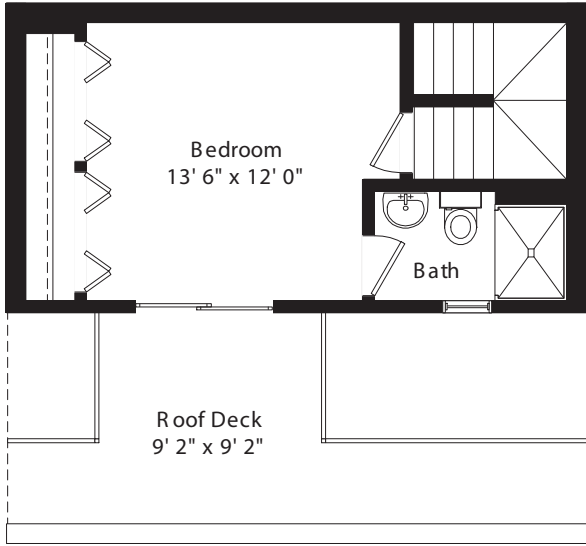
Fourth Floor
