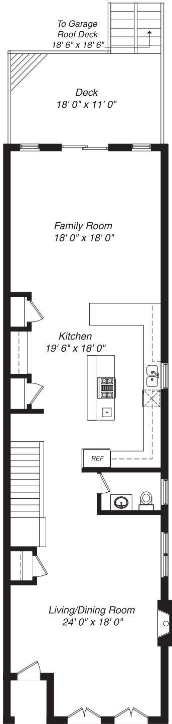
First Floor
