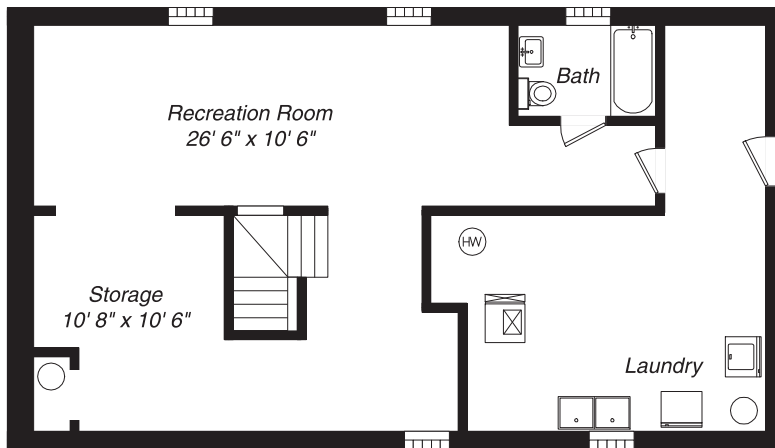
Lower Level
