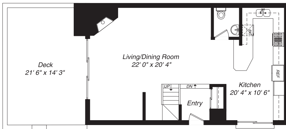
First Floor
