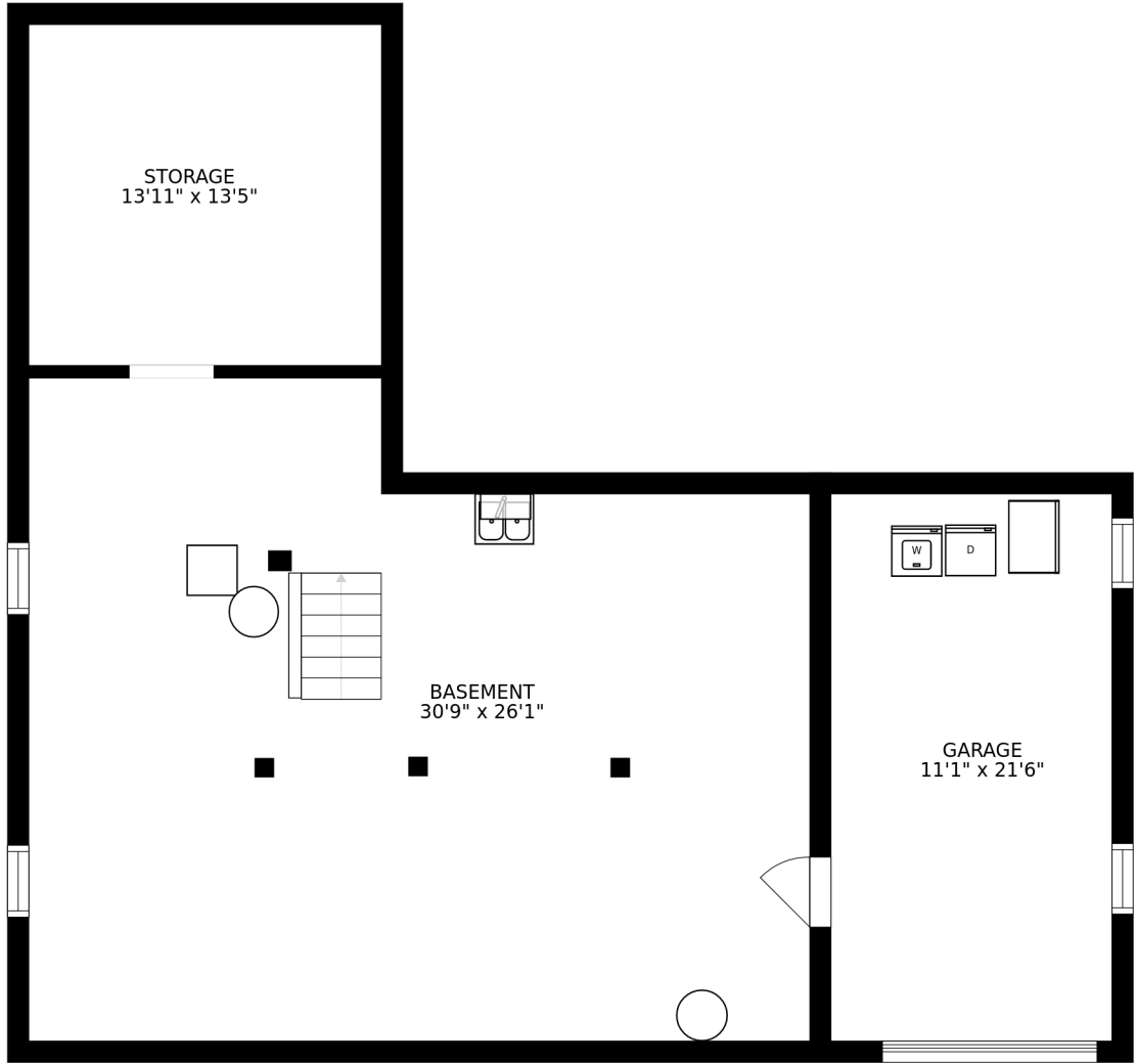
FLOOR 1
