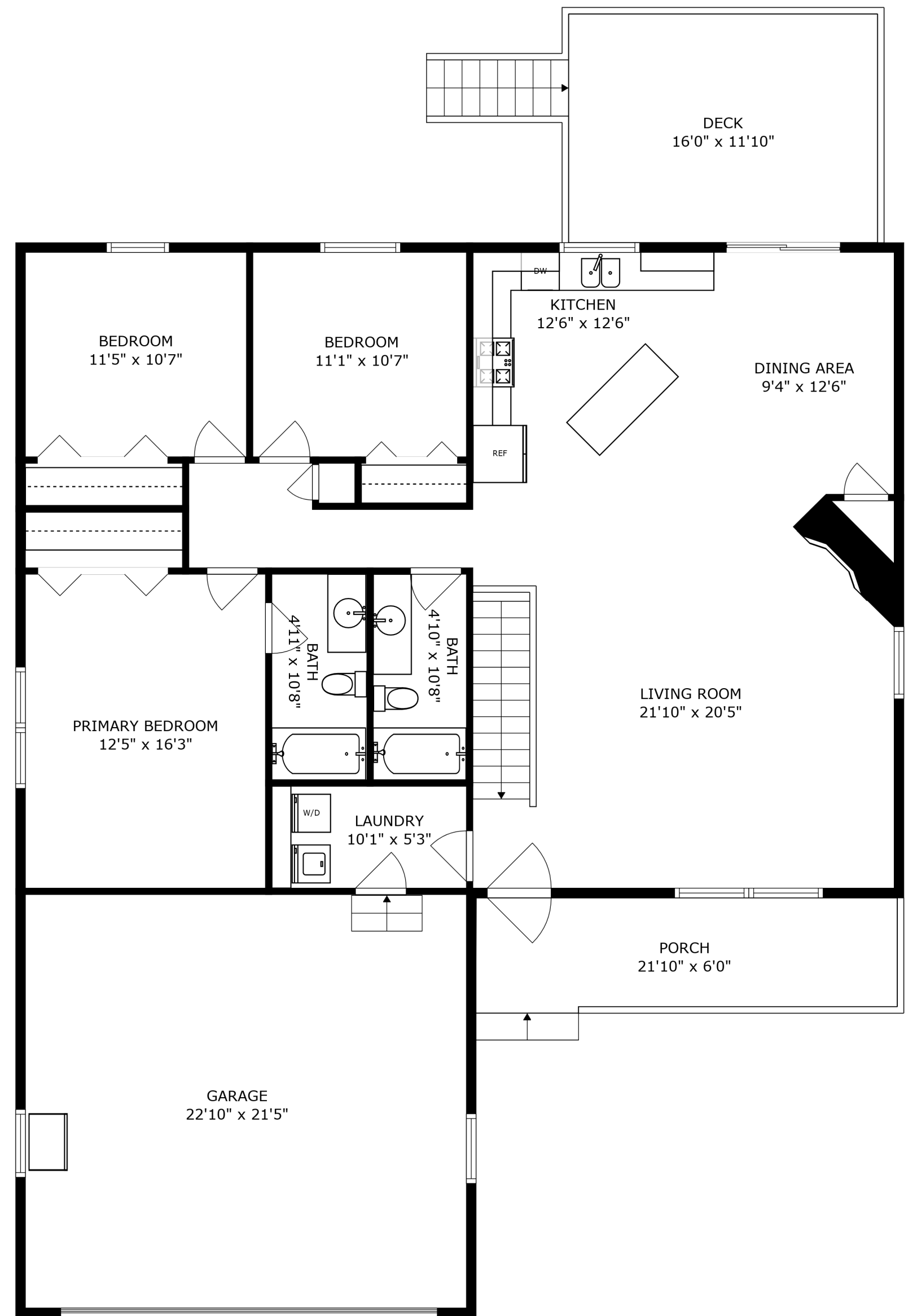
FLOOR 2
