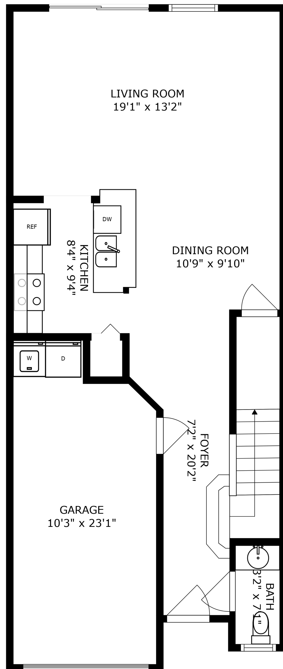
FLOOR 1
