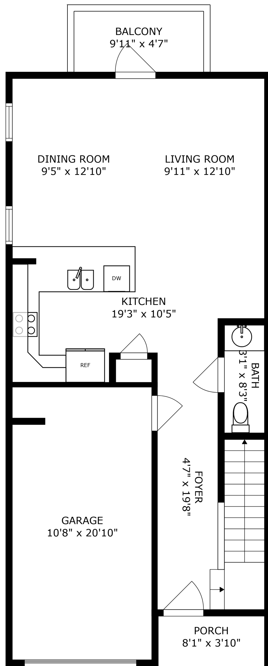
FLOOR 1
