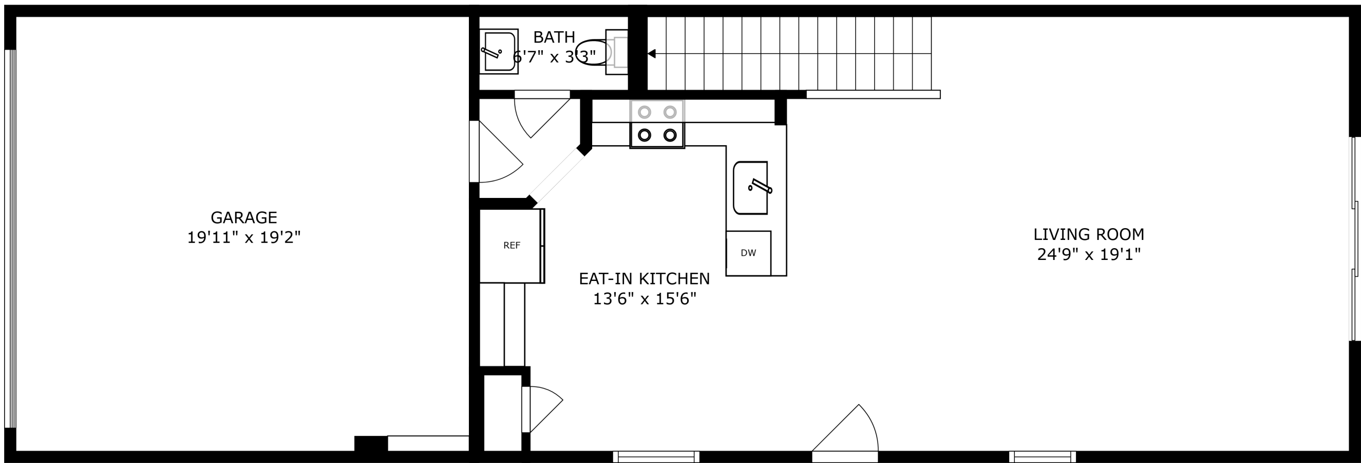
FLOOR 1
