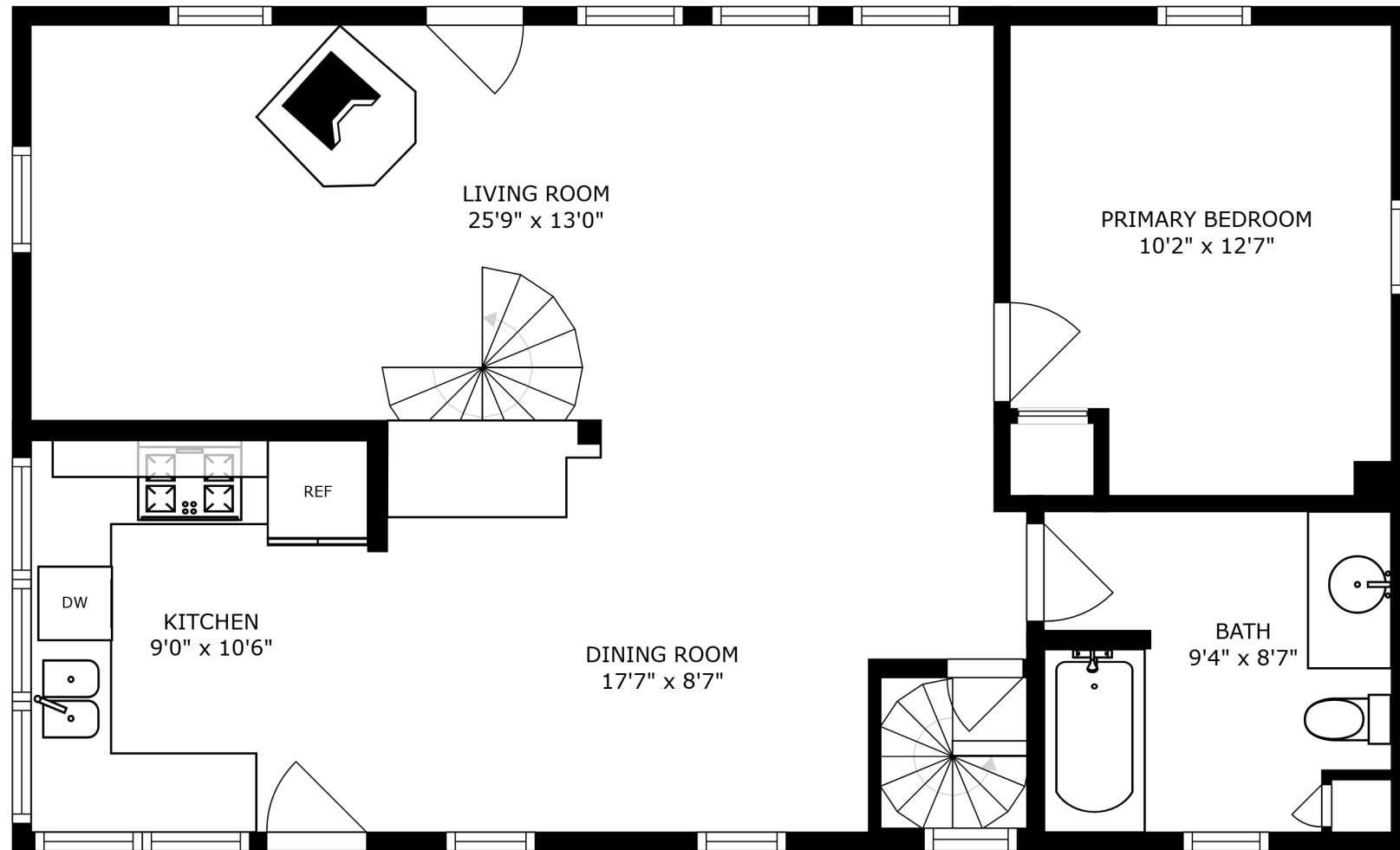
FLOOR 2
