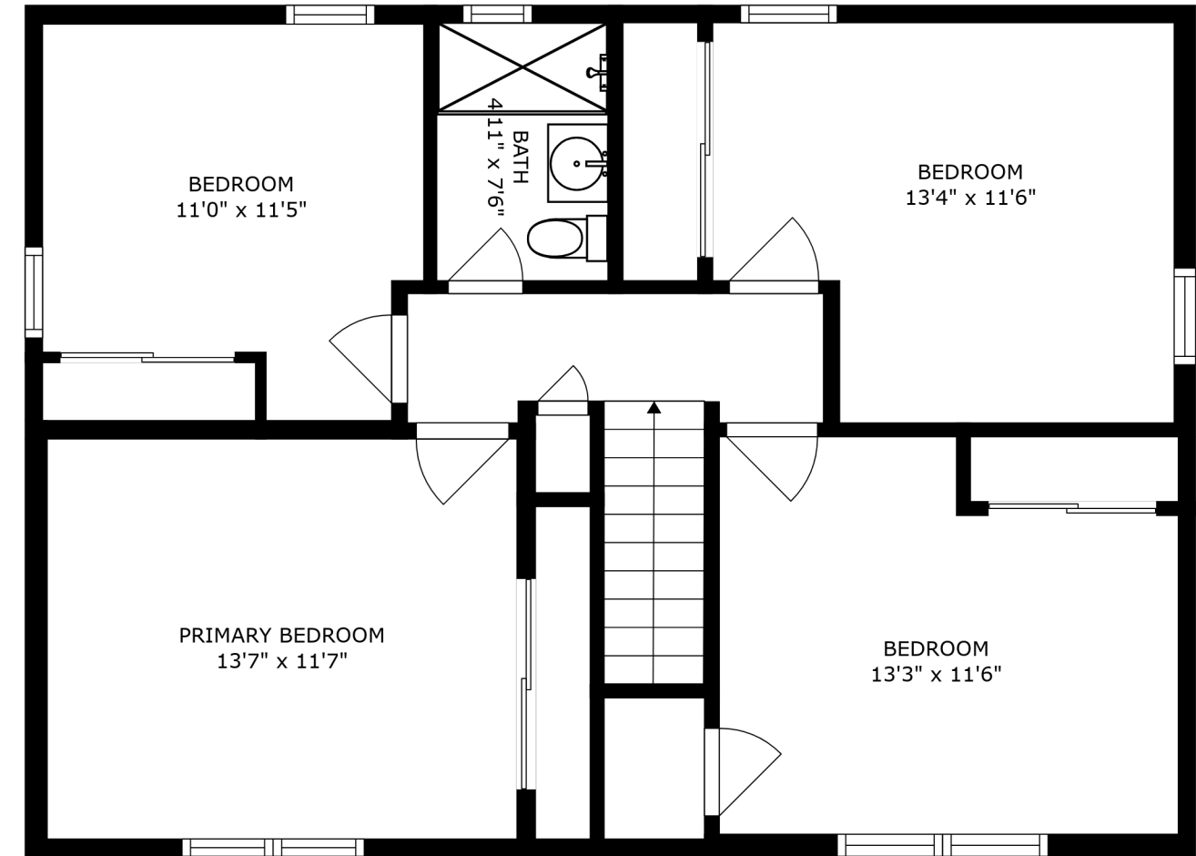
FLOOR 3
