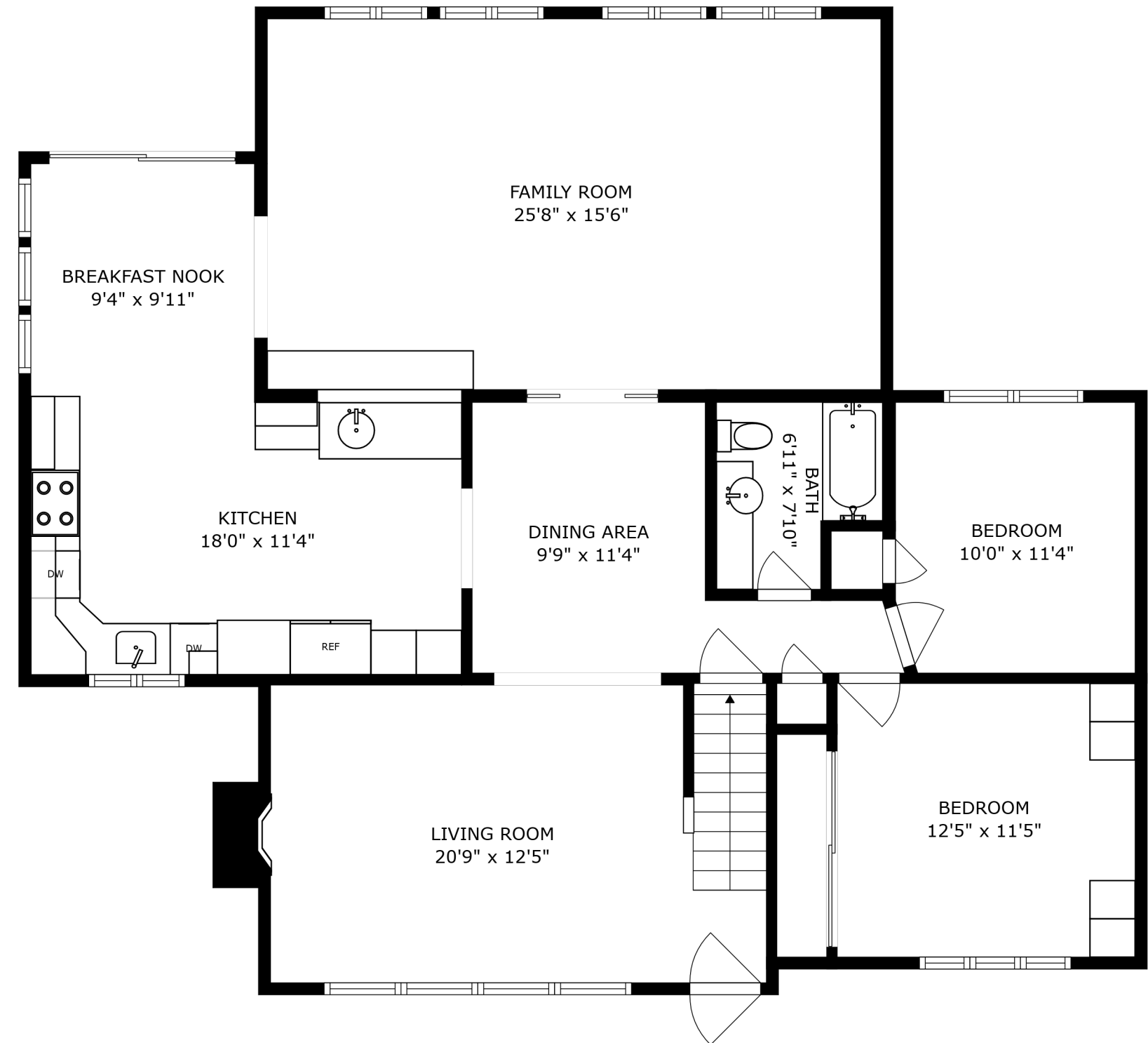
FLOOR 2
