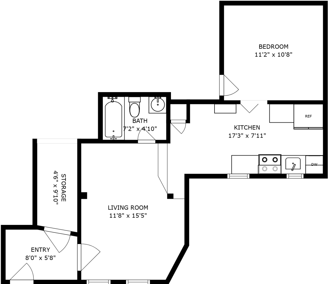
FLOOR 3
