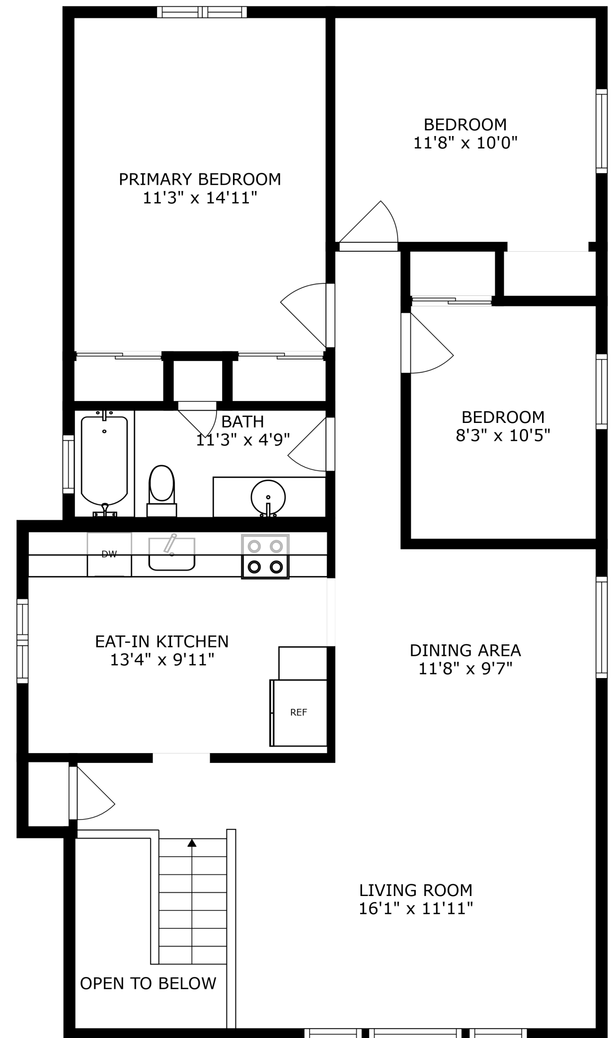
FLOOR 2
