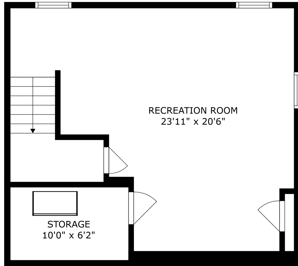
FLOOR 1
