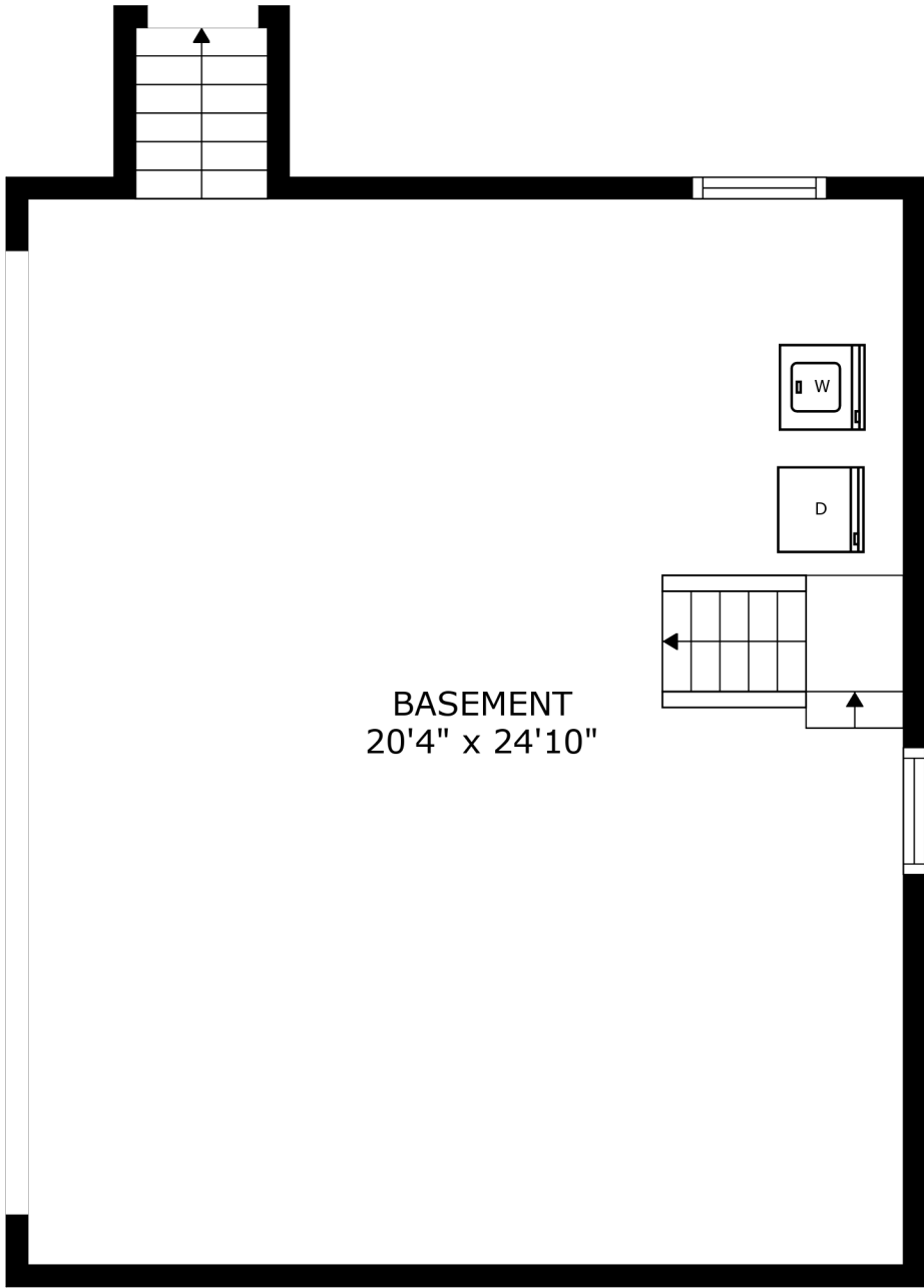
FLOOR 1
