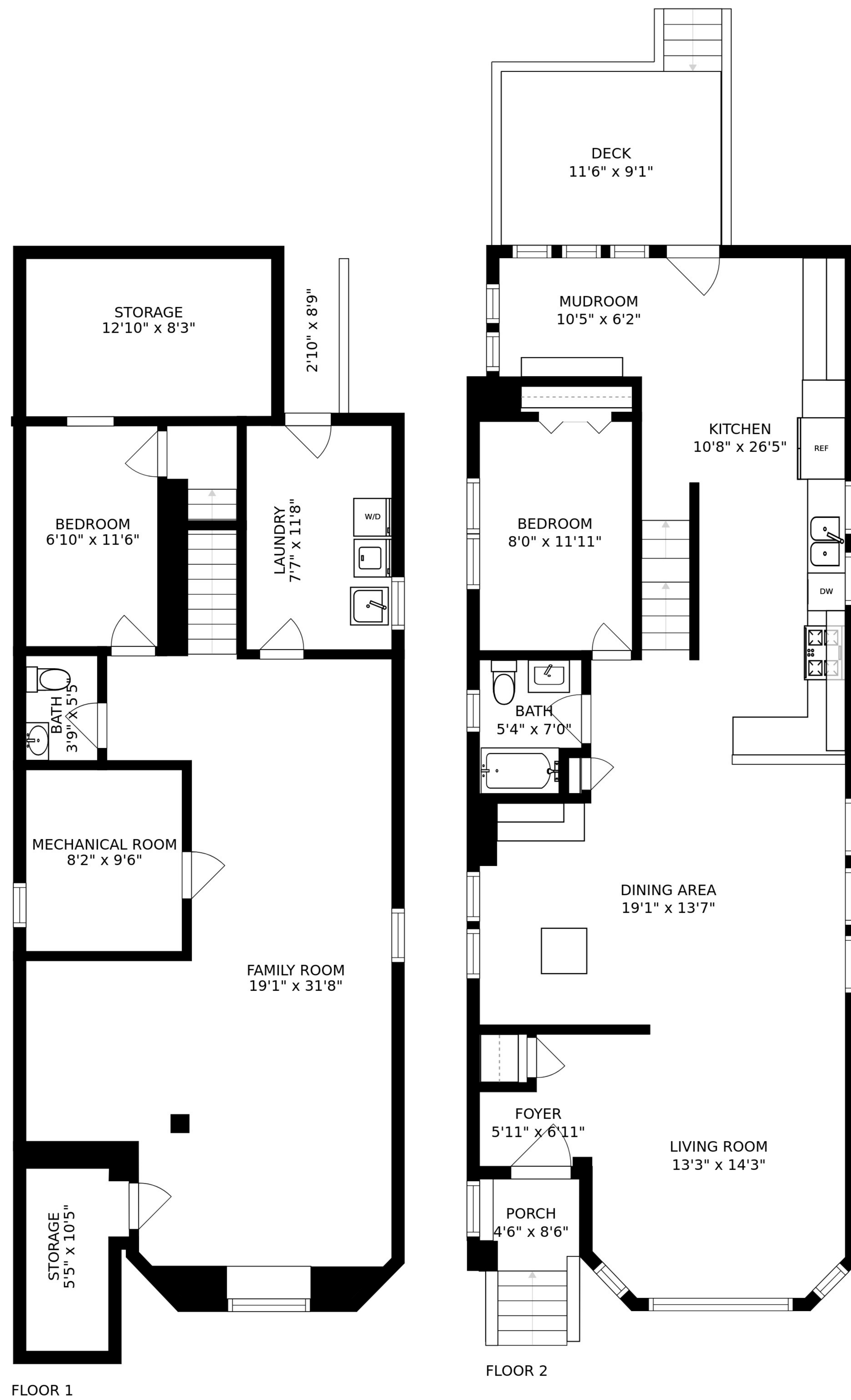
FLOOR 1
